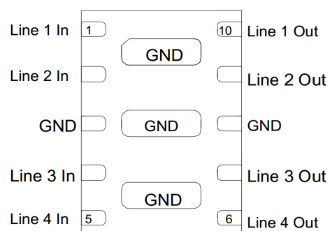
Pin Schematic
