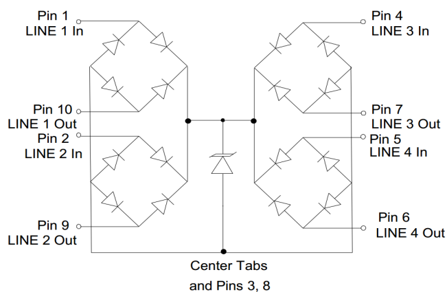
Circuit Schematic
